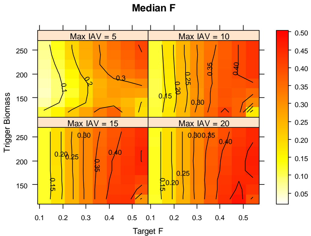
Figure 4.4.1.4. Realised F at scenarios of high recruitment (1991-2006 geometric mean) and low assessment error (CV=10%)
